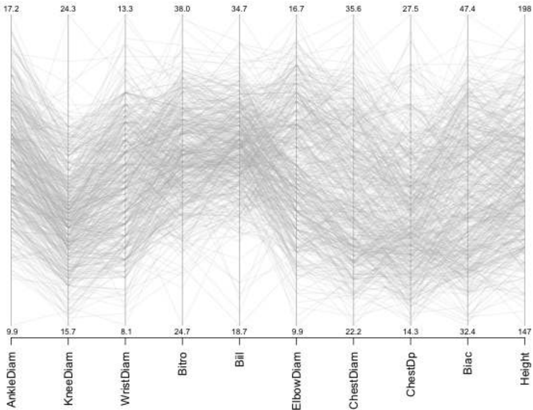
Figure 12: Parallel coordinates of the skel2 data set.
