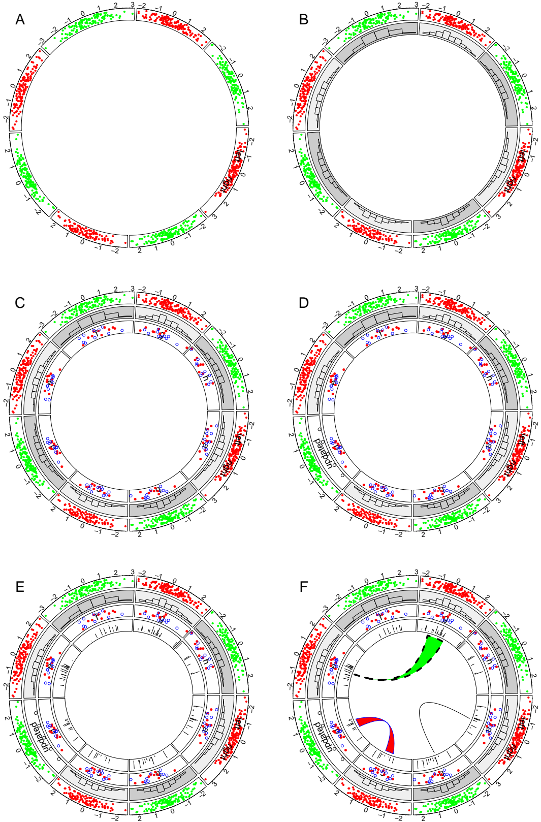
Figure 2: A step-by-step example by circlize .
