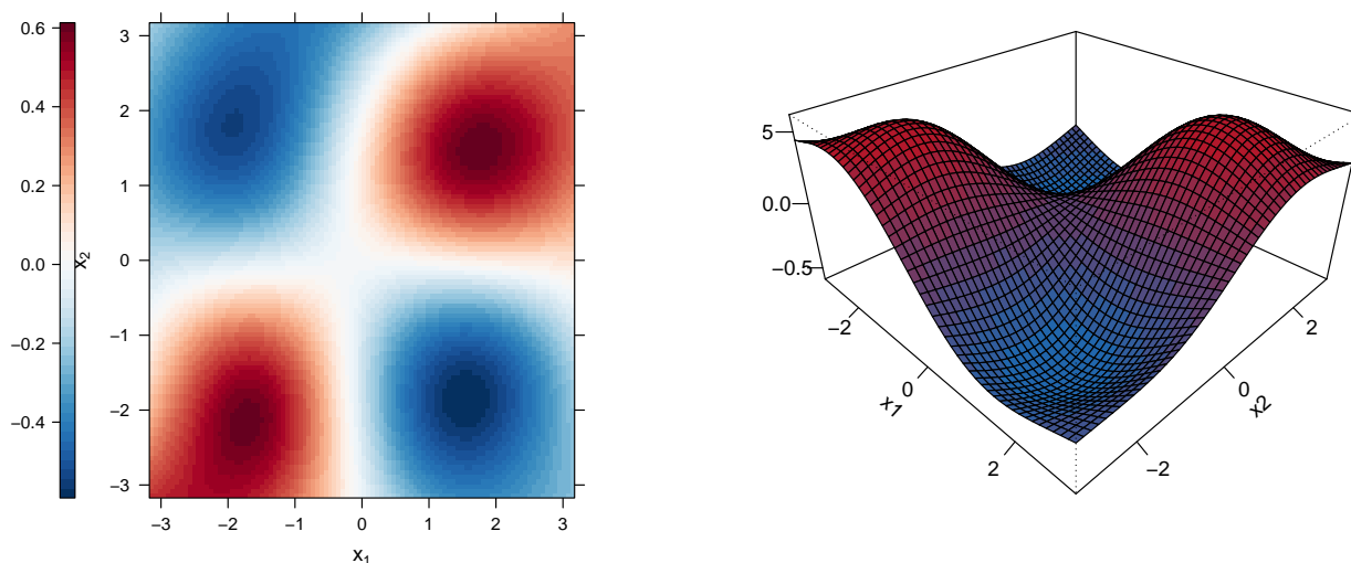
Figure 6: Example for interaction surface fitted using bspacial() . Two displays of the same function estimate are presented (levelplot: left; perspective plot: right). True function: f(x_1, x_2) = \sin(x_1) \cdot \sin(x_2) .
