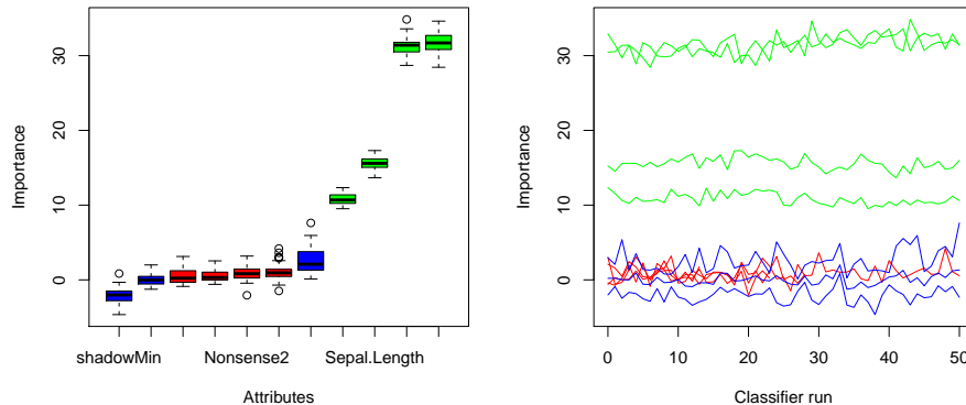
Figure 1: The result of calling plot (left) and plotImpHistory (right) on the BorutaOnIrisE object.
