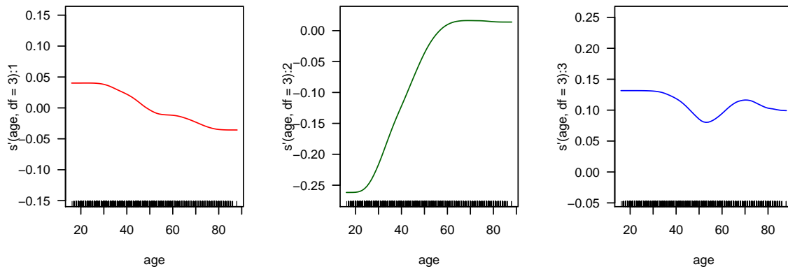
Figure 2: Estimated first derivatives of the component functions, \hat{f}'_{(s)2}(x_2) , from the NZ marital status data (see Equation 14).
