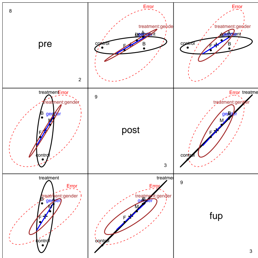
Figure 5: HE plot for the mod1.OBK repeated measures model, showing between-S effects for all pairs of sessions. The panel in row 2, column 1 is identical to that shown separately in Figure 4.
