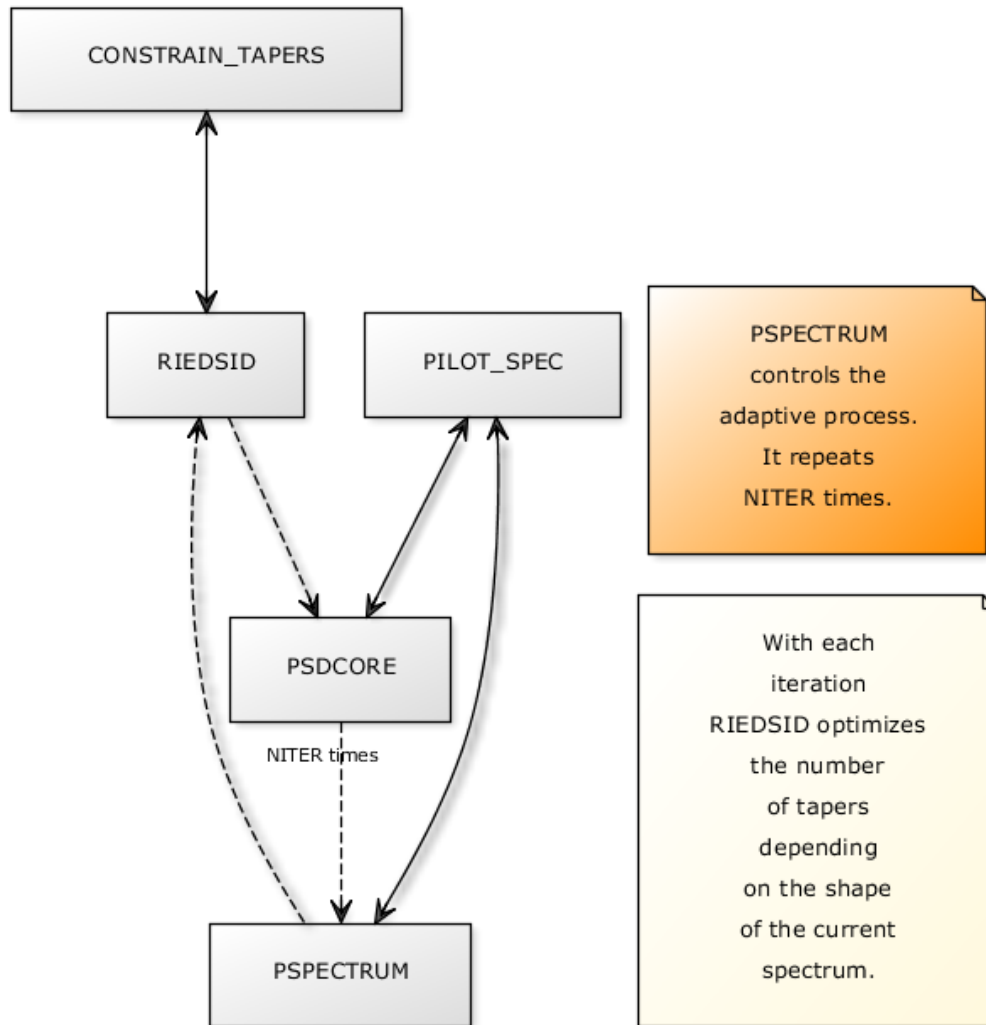
Figure 12: Simplified call graph for pspectrum . The dashed lines show a simplified circuit which the spectra and its tapers make during the iterative process.
