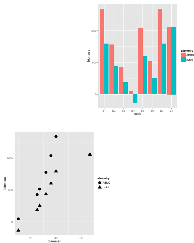
Figure 3: Bar plot and dot plot comparing biomass estimates of allometryABDC and allometryCutini2009 functions to stonePine2FieldData
